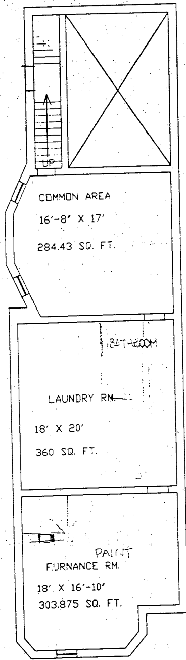
BASEMENT FLOOR PLAN 405 HURON ST. 96-403
