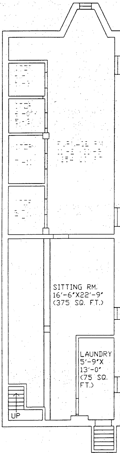
BASEMENT FL. PLAN
