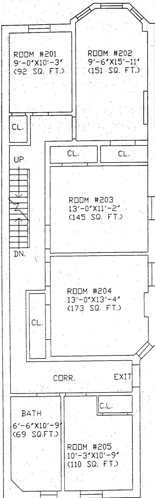
SECOND FL. PLAN
